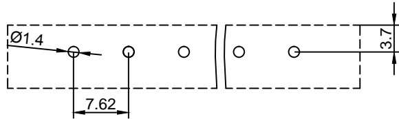
PCB Layout
